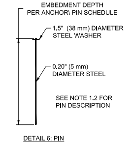
DETAIL 6: PIN
