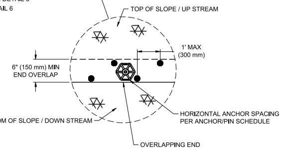
DETAIL 4: PIN PATTERN AND OVERLAPS
