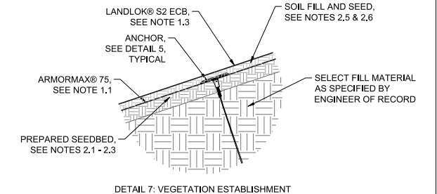
DETAIL 7: VEGETATION ESTABLISHMENT
