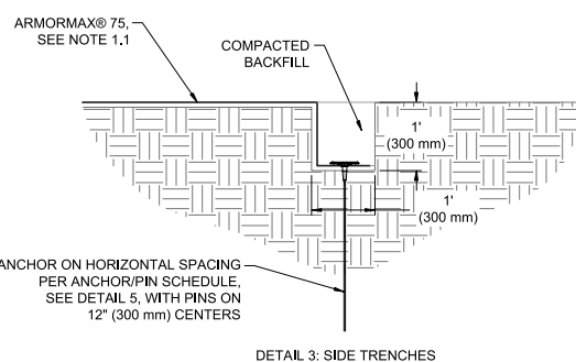
DETAIL 3: SIDE TRENCHES
